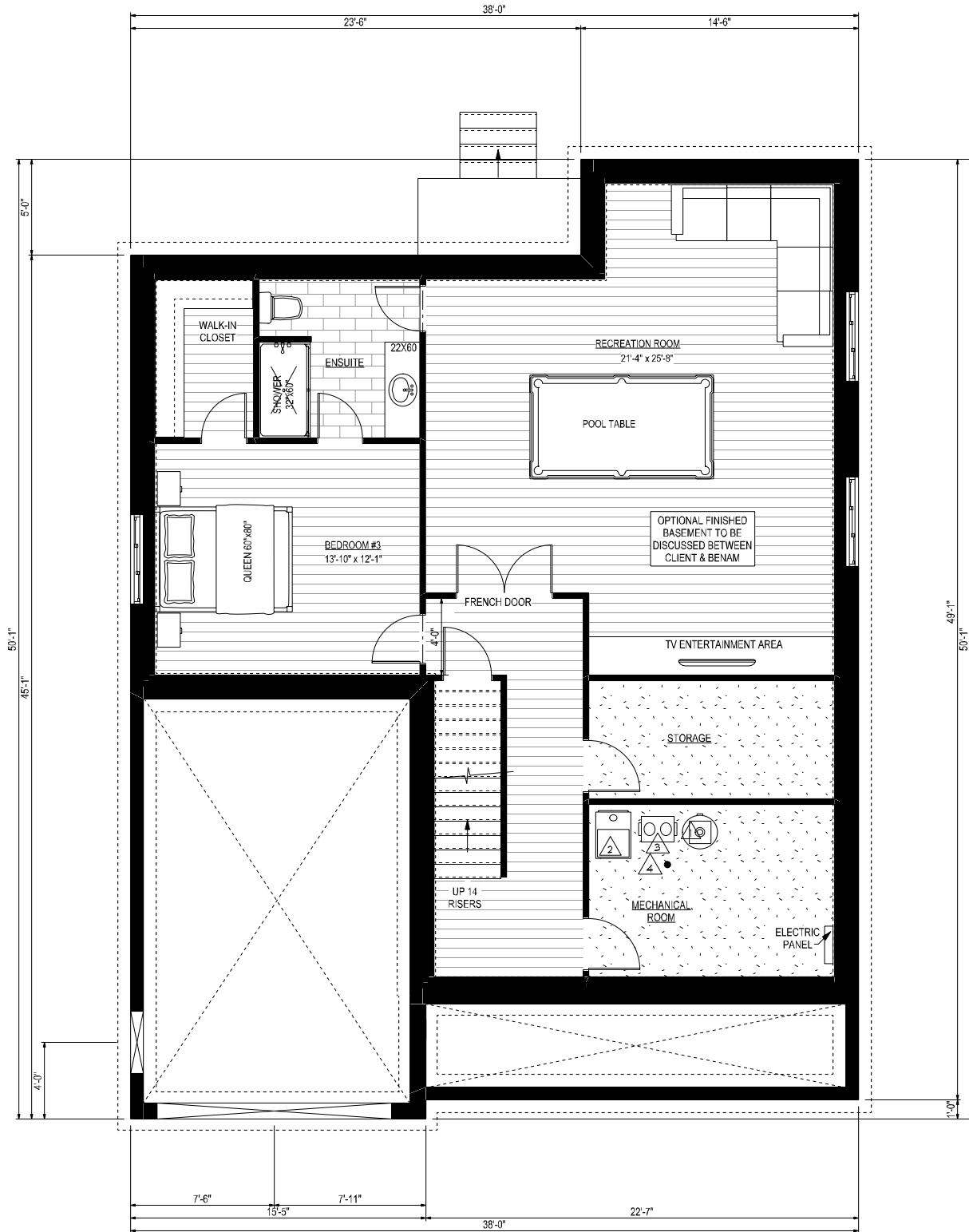
FOUNDATION PLAN
