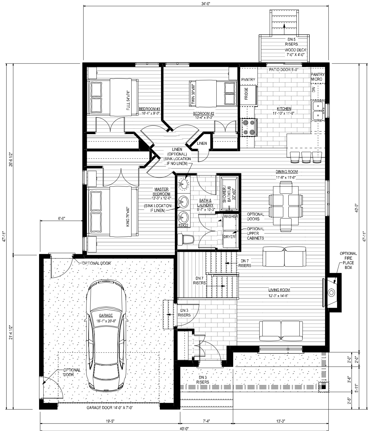
MAIN FLOOR PLAN (3 BEDROOM)
