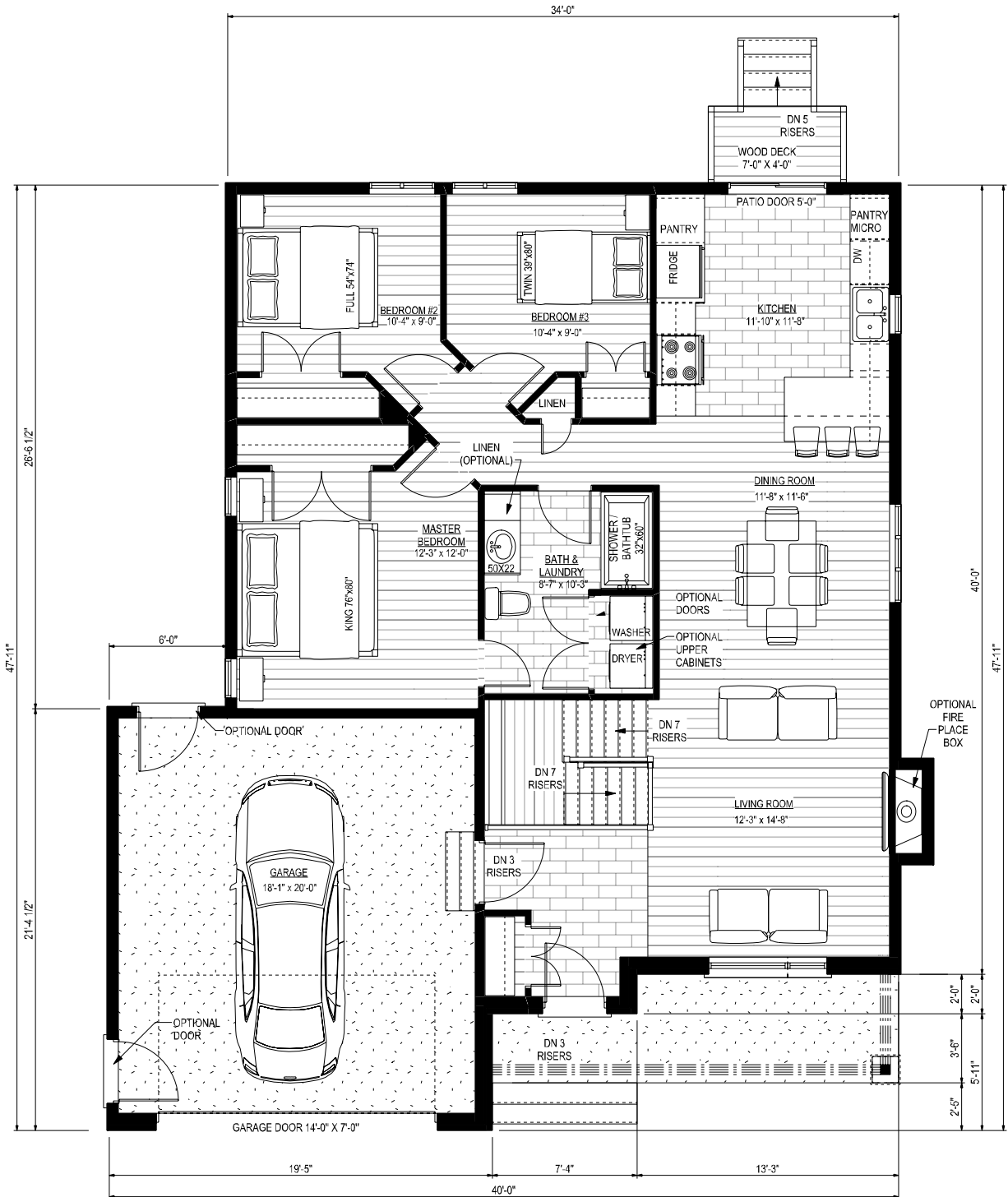
MAIN FLOOR PLAN (3 BEDROOM) (CHEATER ENSUITE)
