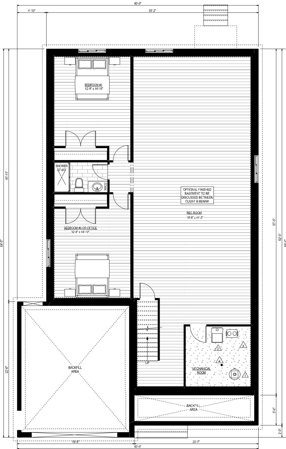
FOUNDATION / BASEMENT PLAN
