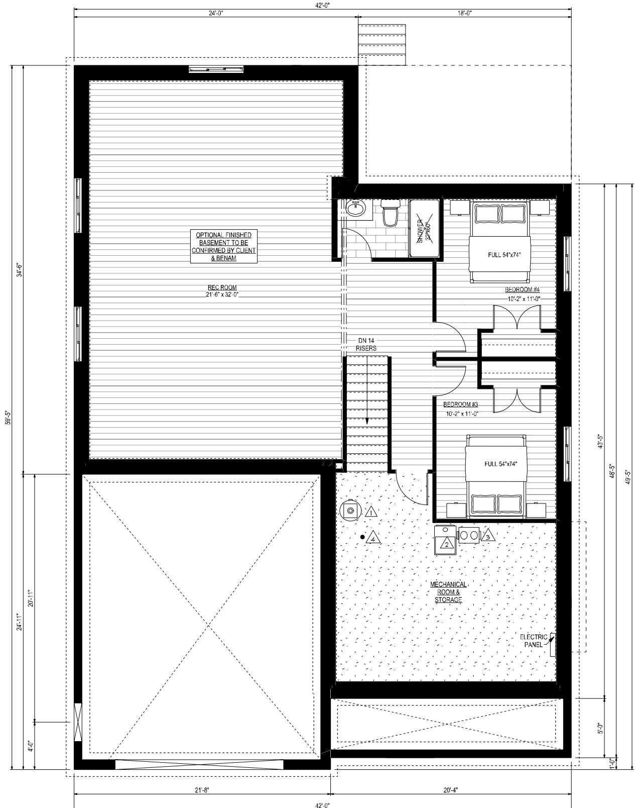
FOUNDATION / BASEMENT PLAN
