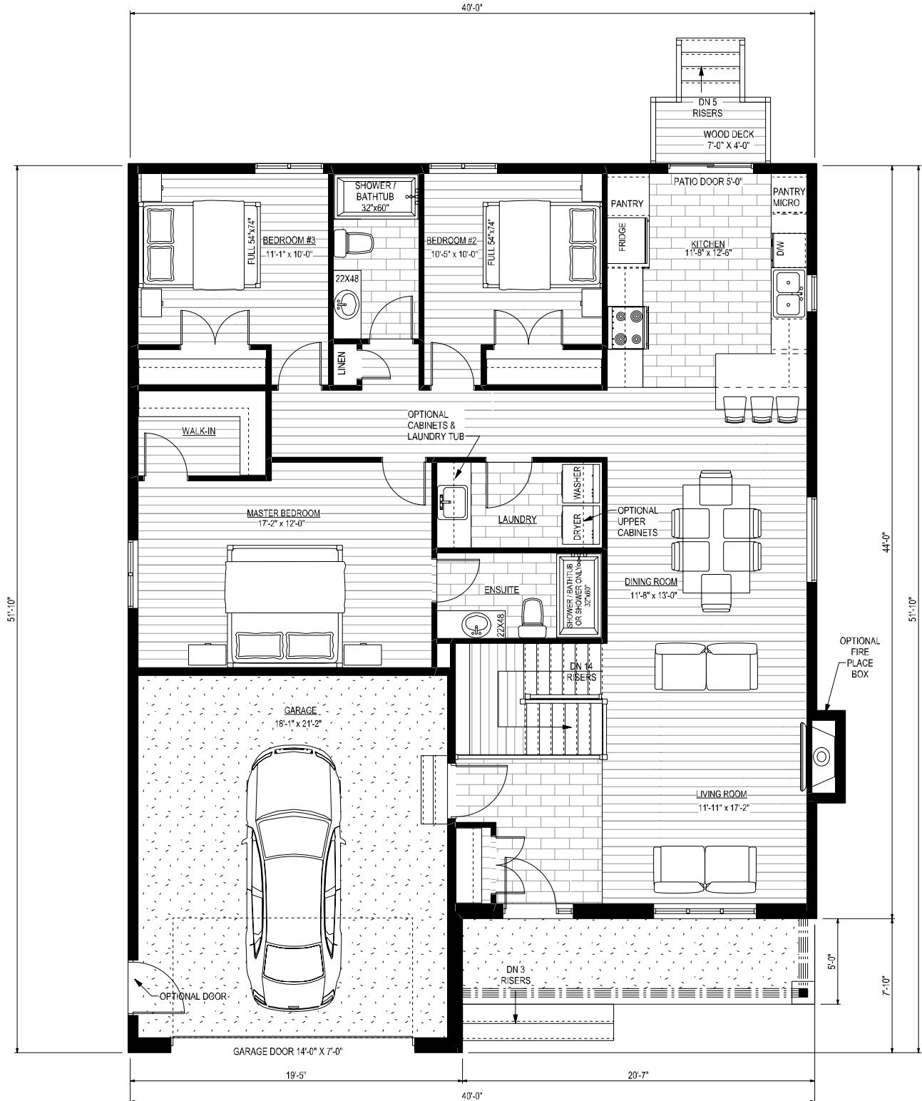
MAIN FLOOR PLAN (3 BEDROOM)
