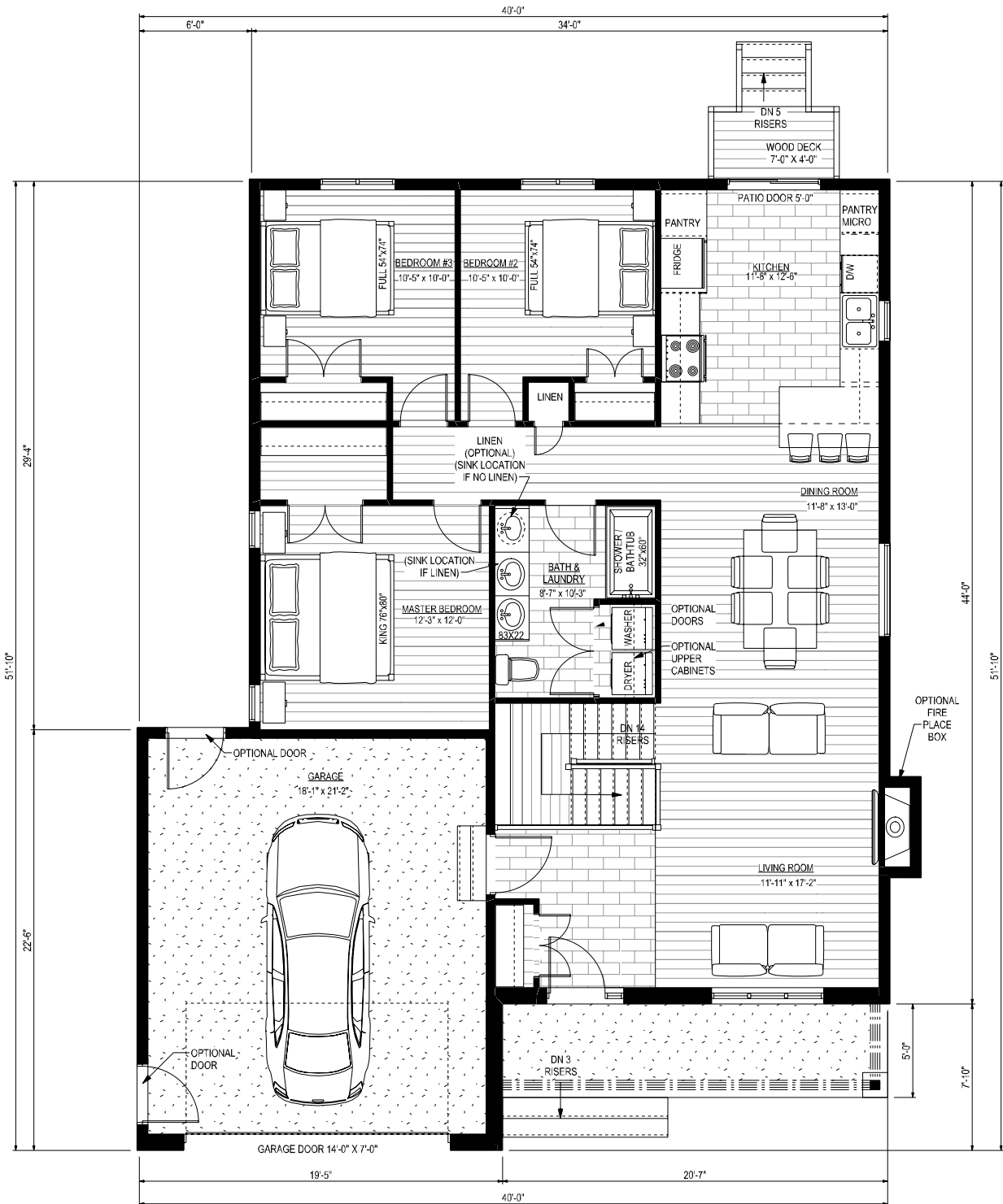
MAIN FLOOR PLAN (3 BEDROOM)
