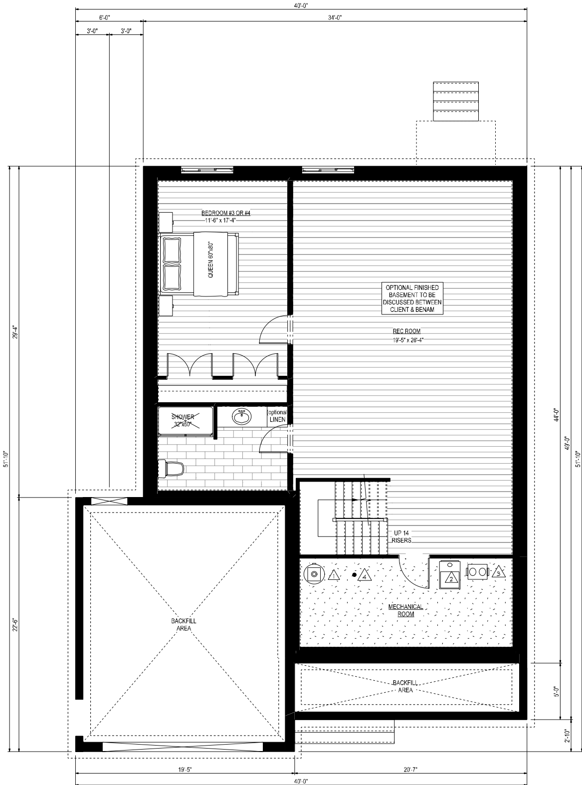
FOUNDATION / BASEMENT PLAN
