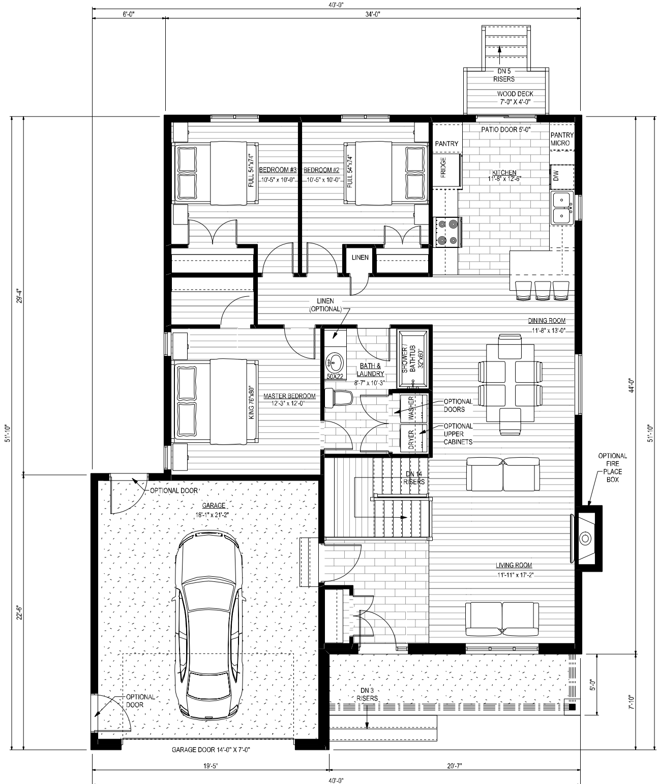
MAIN FLOOR PLAN (3 BEDROOM) (CHEATER ENSUITE)
