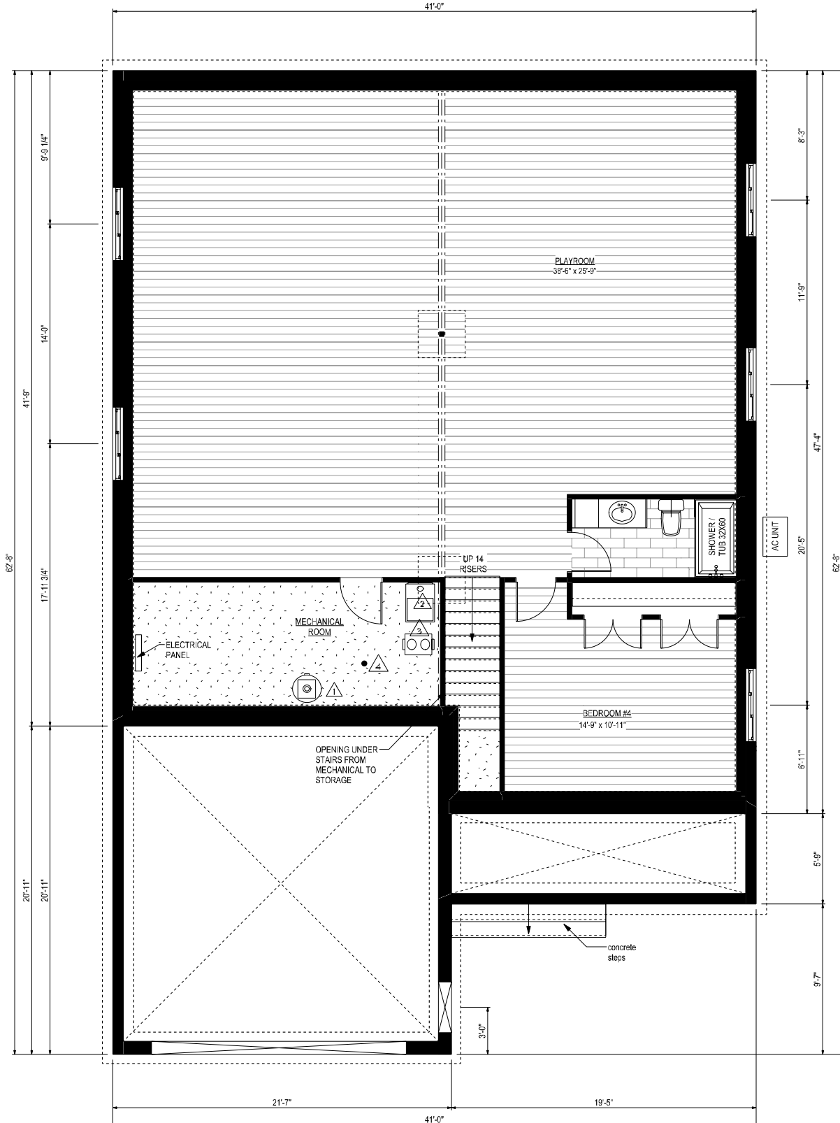
FOUNDATION / BASEMENT PLAN
