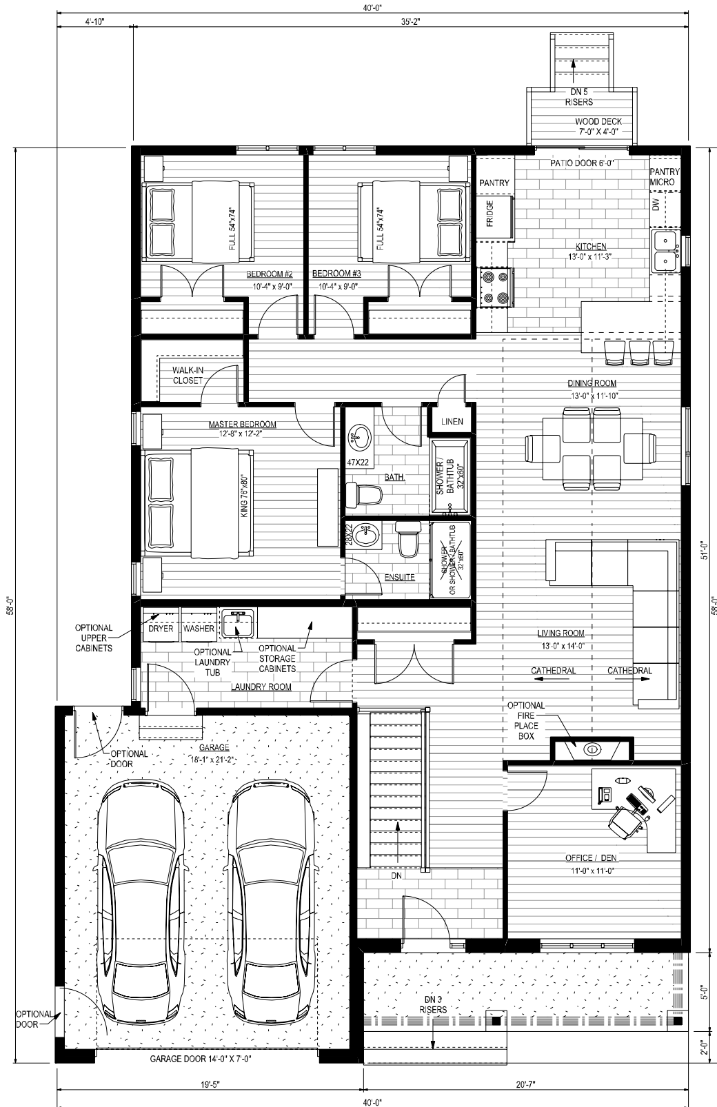
MAIN FLOOR PLAN (3 BEDROOM)
