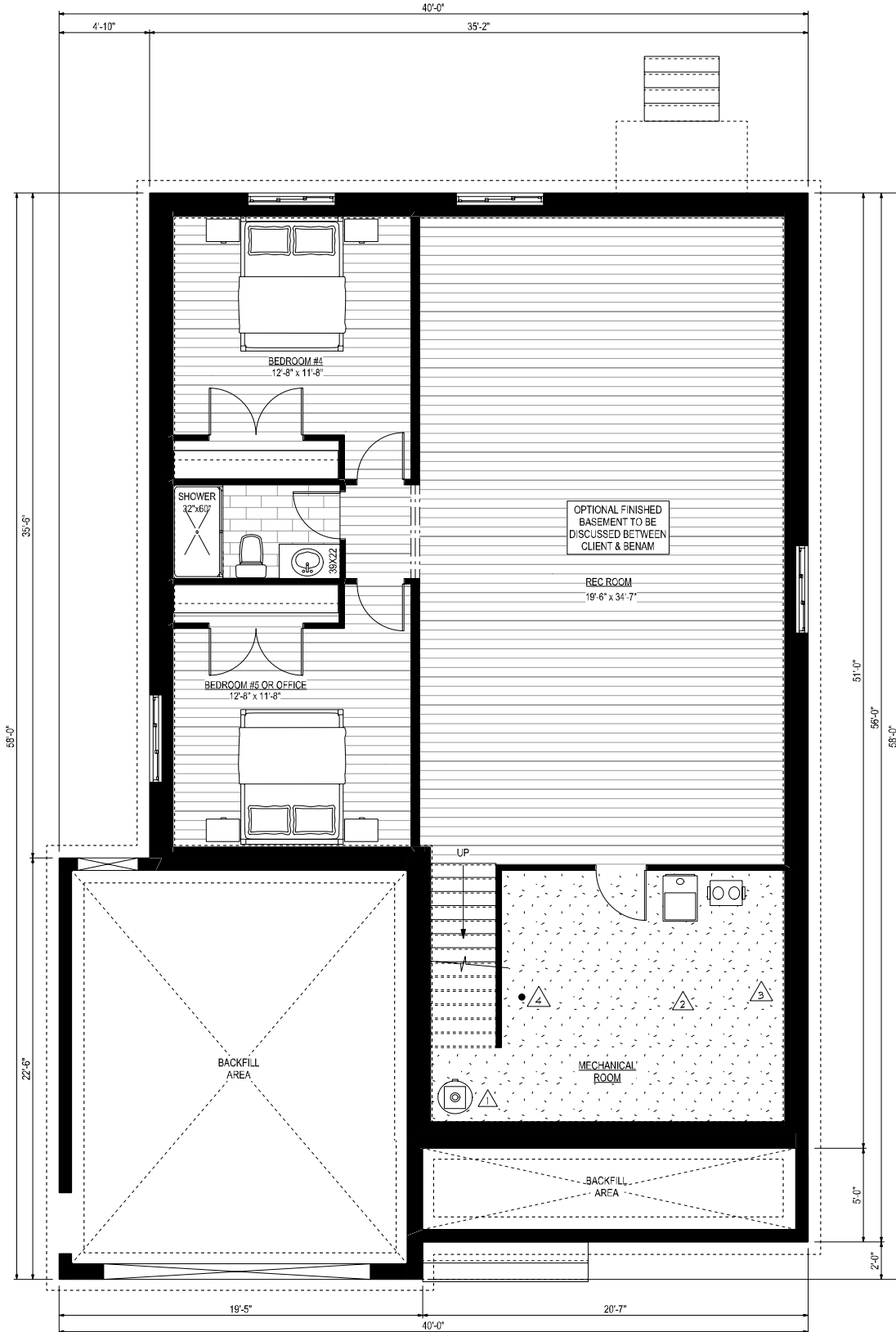
FOUNDATION / BASEMENT PLAN
