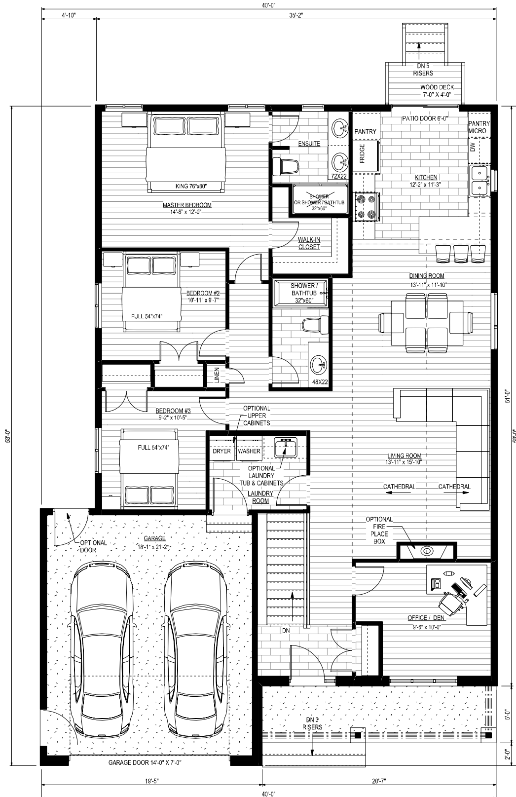
MAIN FLOOR PLAN (3 BEDROOM) (MASTER BED REAR)
