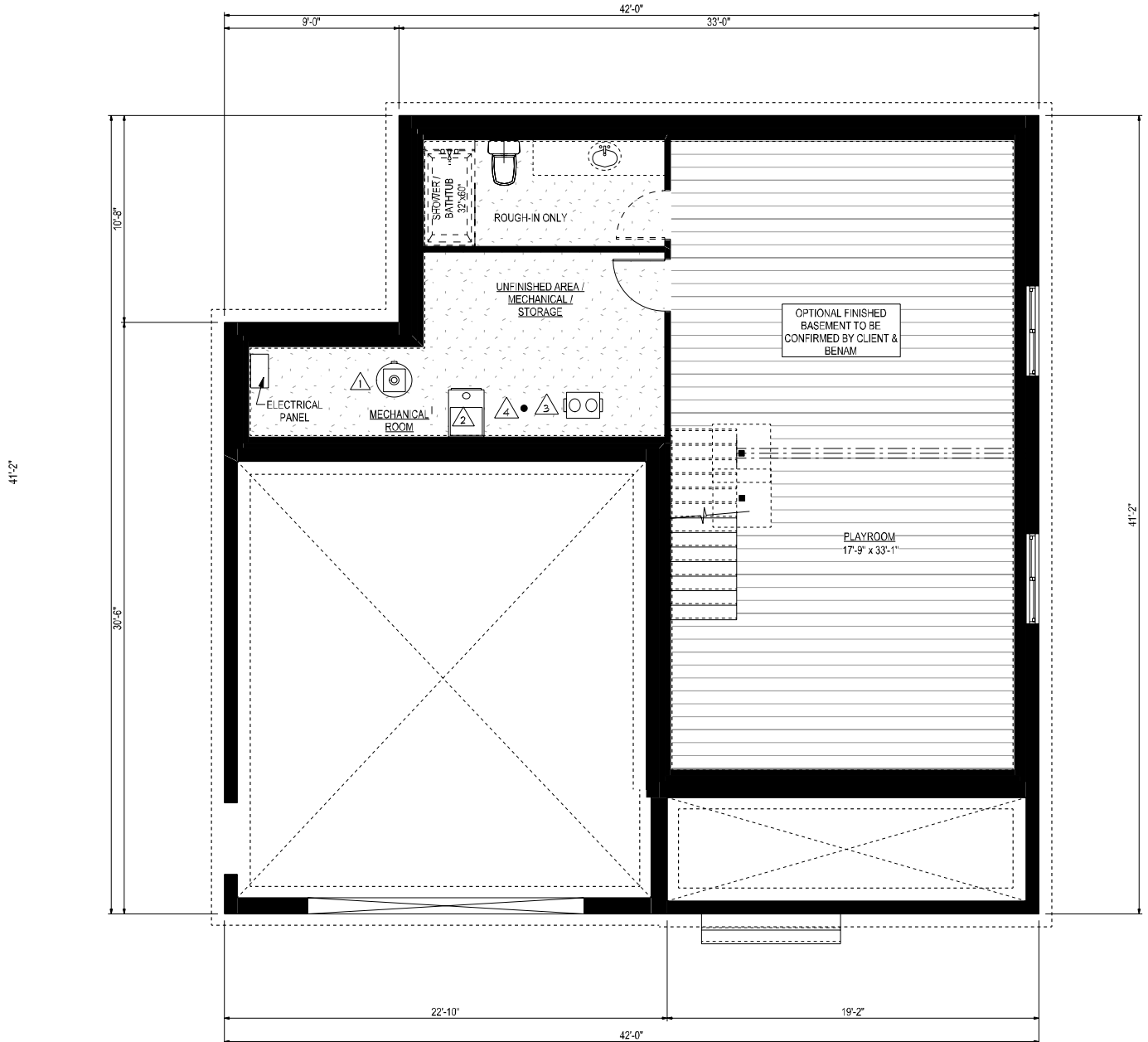
FOUNDATION / BASEMENT PLAN
