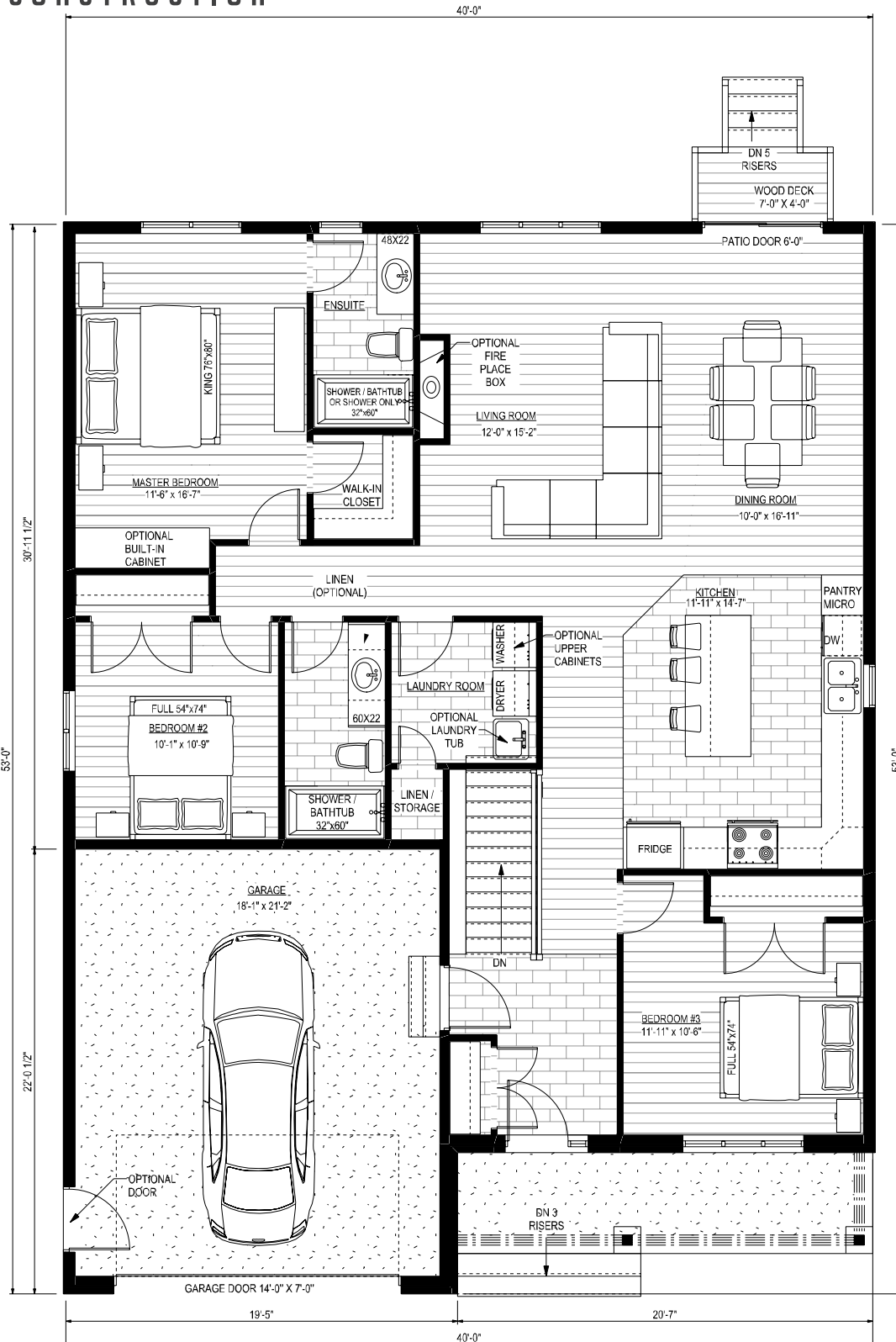
MAIN FLOOR PLAN (3 BEDROOM)
