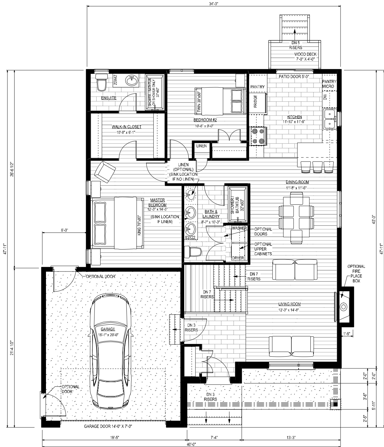
MAIN FLOOR PLAN (2 BEDROOM)
