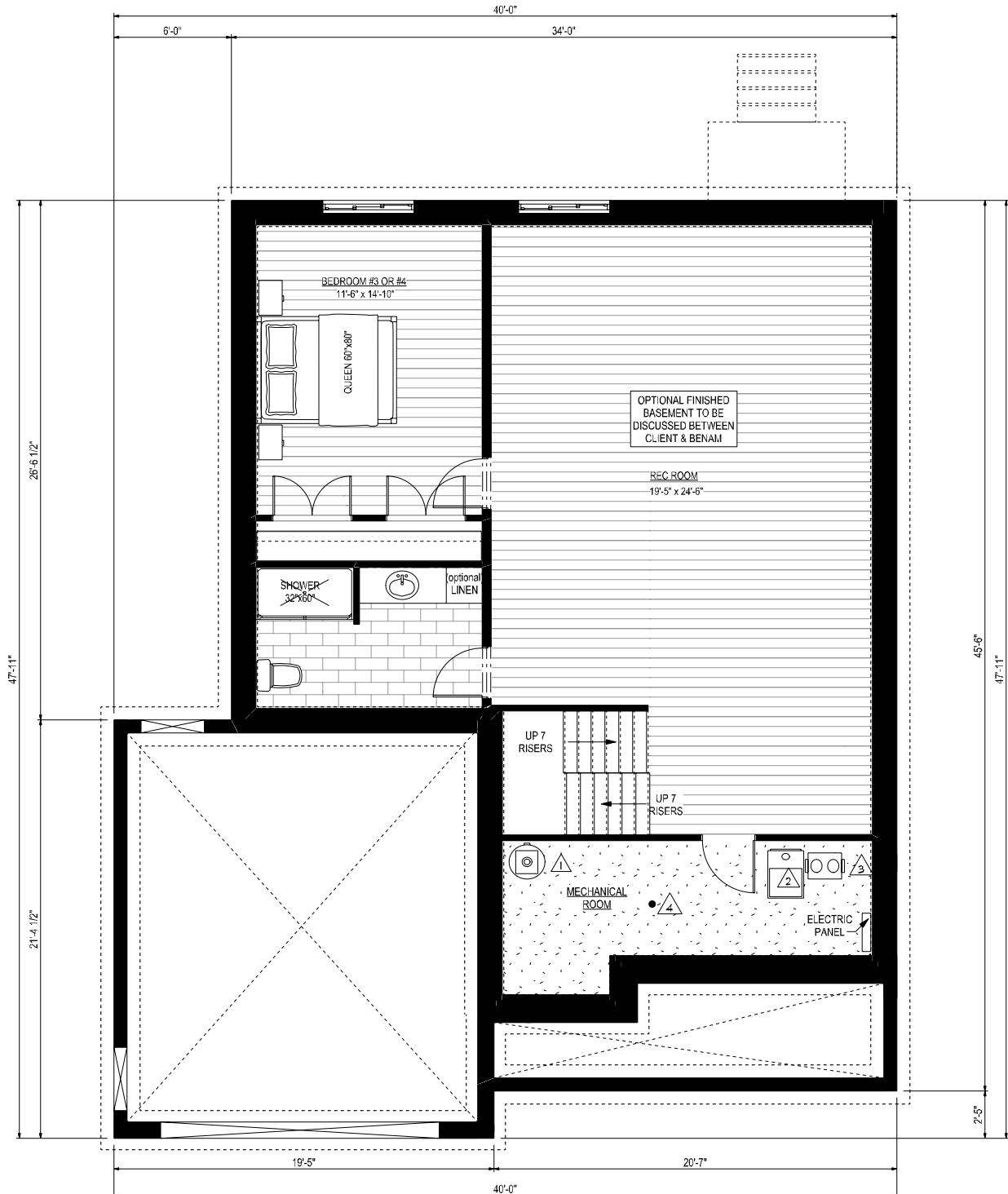
FOUNDATION / BASEMENT PLAN
