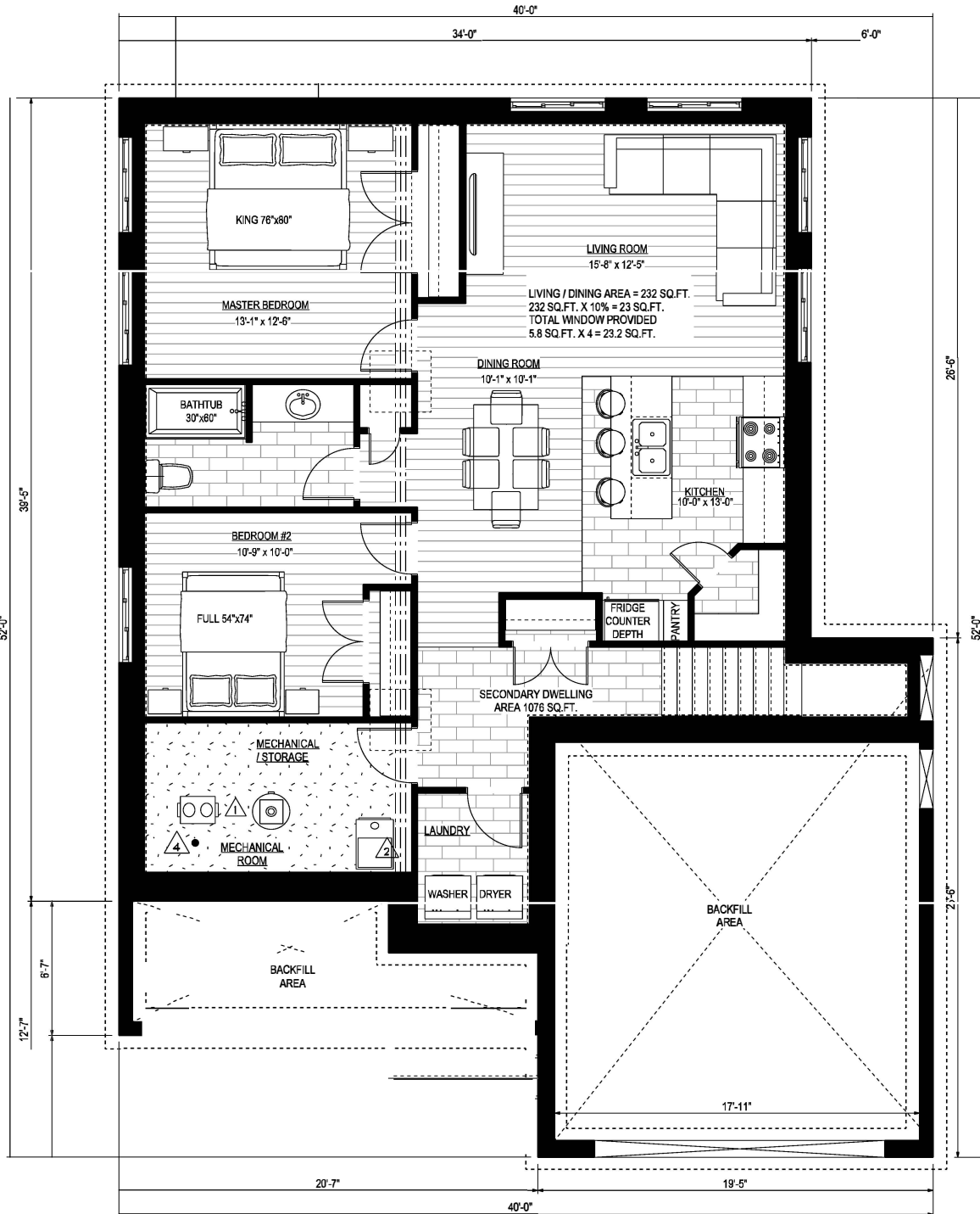
BASEMENT PLAN
